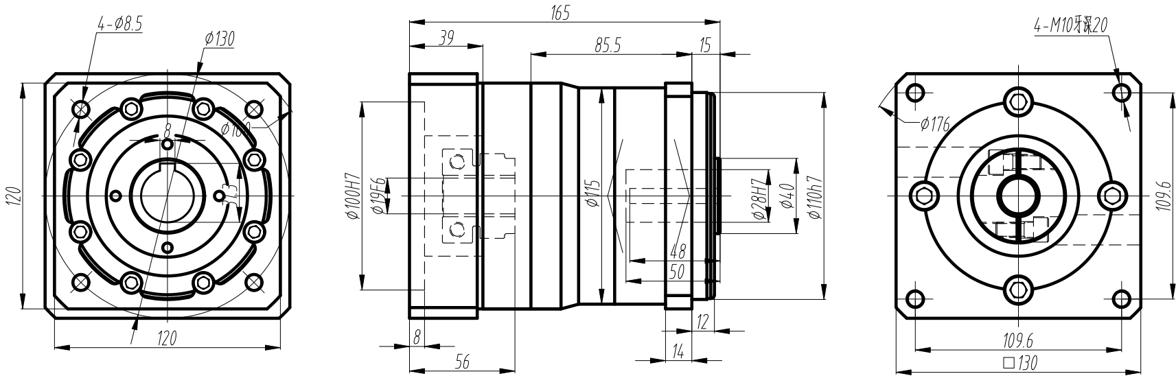
标准轴 Standard output shaft
